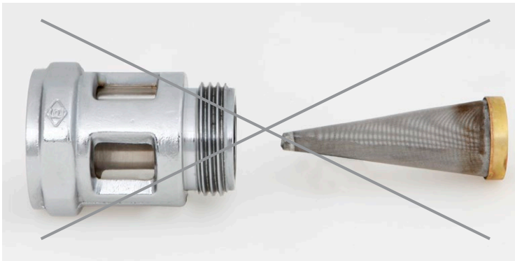
ALT: SG 1" cr mit Feinsieb (Spitzsieb) 160 my aus Edelstahl OLD: SG 1" cr with fine screen (cone shaped) 100 mesh of stainless steel
