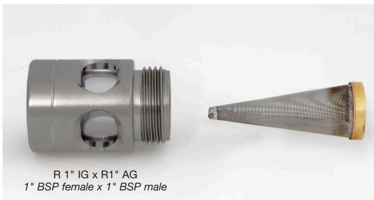
NEU: SG 1" 1 x 0 AI mit Feinsieb (Spitzsieb) 160 my aus Edelstahl NEW: SG 1" 1 x 0 AI with fine screen (cone shaped) 100 mesh of stainless steel
