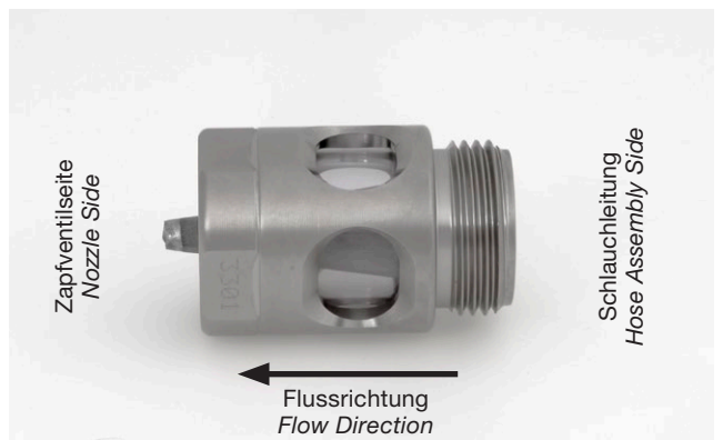
NEU: SG 1" 1 x 0 AI mit Feinsieb (Spitzsieb) 160 my aus Edelstahl NEW: SG 1" 1 x 0 AI with fine screen (cone shaped) 100 mesh of stainless steel
