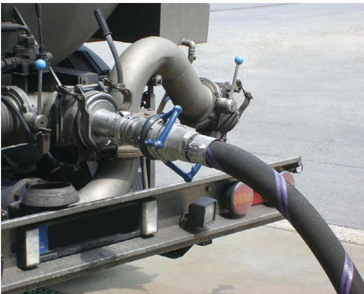
FEP universal hoses / filling IBC with chemicals - Storck, Germany
