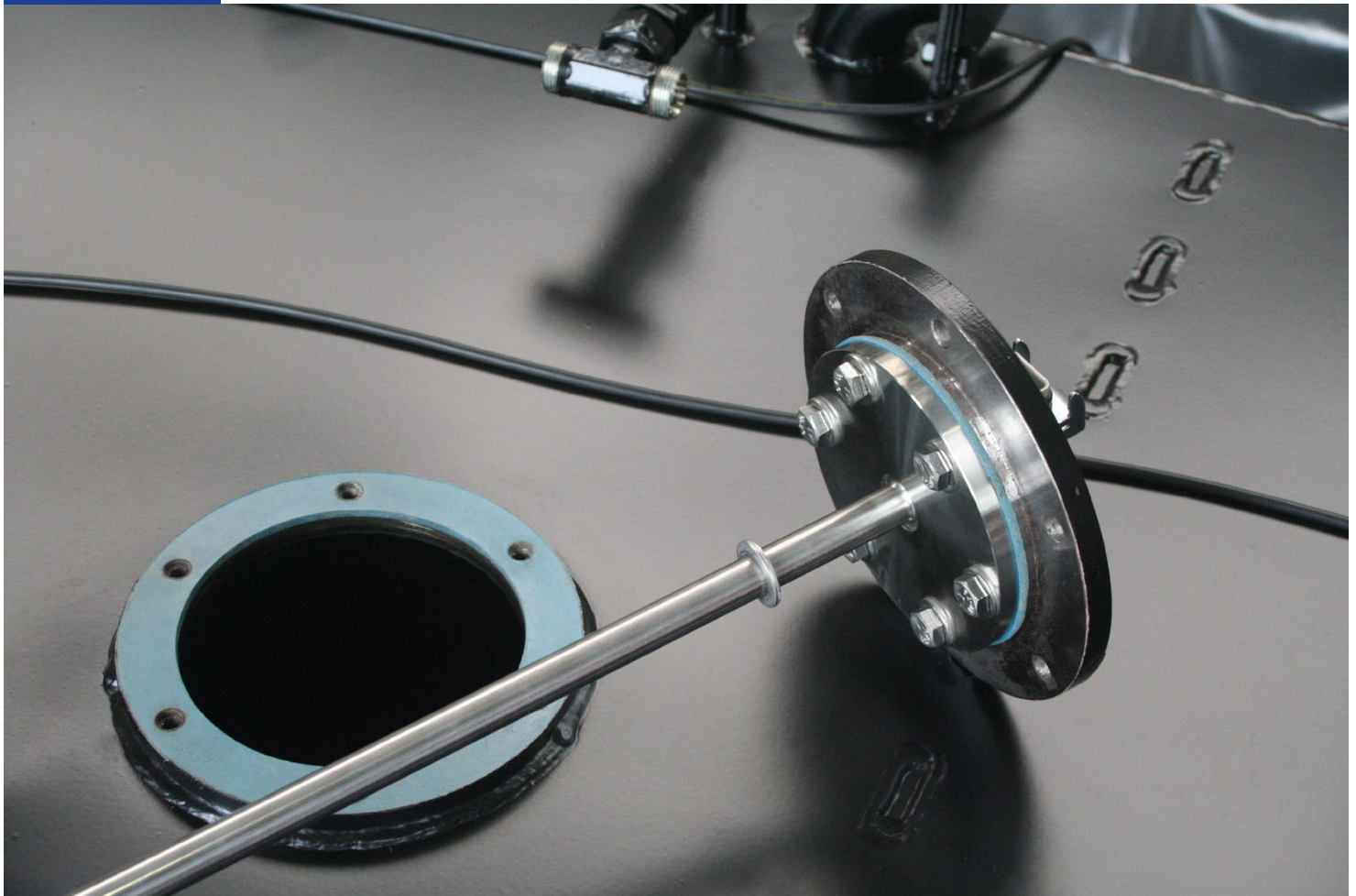
ELAPAC seals / locomotive tanks - Burmann Dichtungstechnik, Germany
