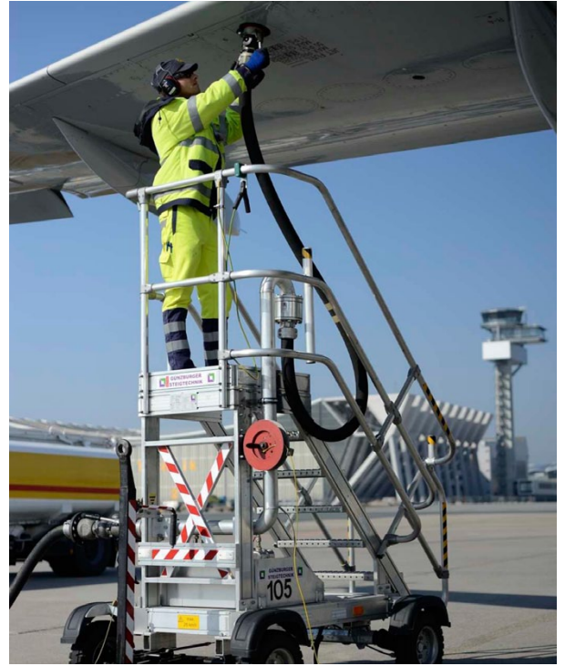
HD-C / underwing refuelling - Frankfurt Jet Services, Germany
