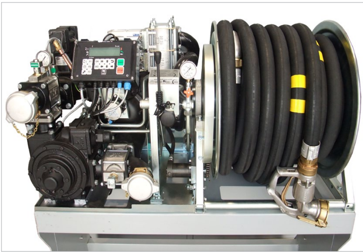
ZV 400 + HD reel hose / modular dispensing and measuring system for tankers, 700 l/min - Medicion, Spain
