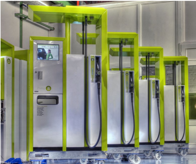
ZVA SL 2 + Slimline hoses / Clou dispensers, last production step - Scheidt & Bachmann, Germany
