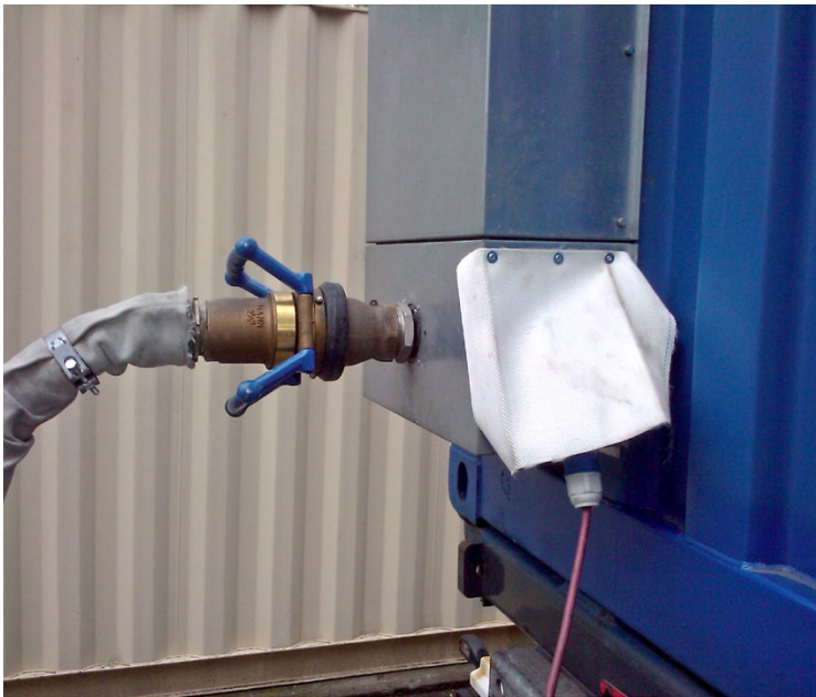
HD 100 Neon spiral / large aerosol canon to avoid dust spreading in mining and deconstruction - Ecology SRL, Italy
